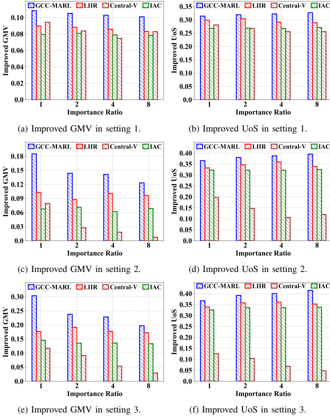
Figure 6: Improved GMV and UoS of different algorithms.
