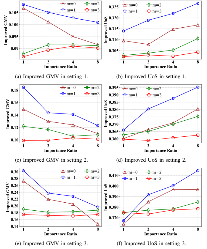
Figure 7: Improved GMV and UoS of GCC-MARL with m \in \{0, 1, 2, 3\} .
