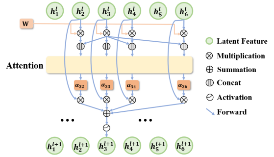
Figure 4: The computation process of the l th GAT layer on node v_3 . The input graph is \mathcal{C}_t^{3,1} based on the reachability graph in Fig. 3b.
