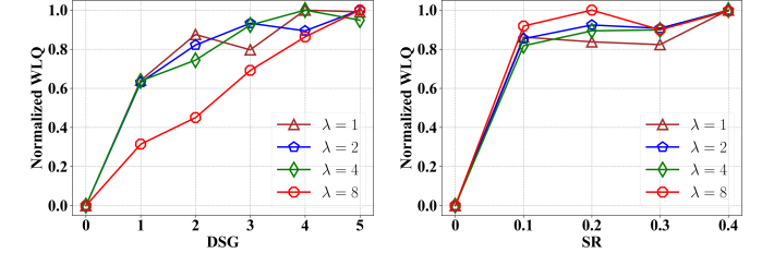
Figure 8: Visualization of Normalized WLQ.
