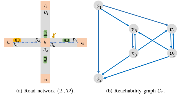
Figure 3: An example of transforming road network into reachability graph.
