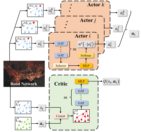
Figure 2: The GCC-MARL framework.
